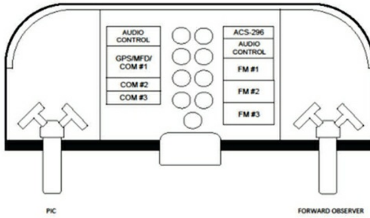
EXHIBIT 4 - PREFERRED PANEL CONFIGURATION
